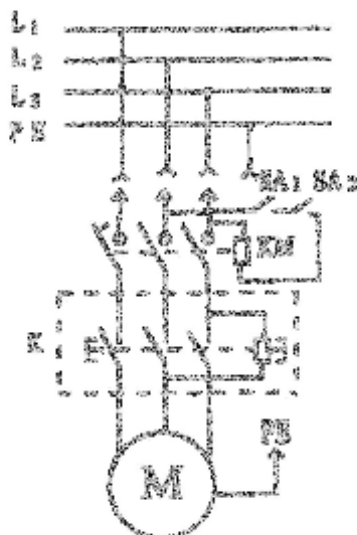
Wire Diagram, three phase, with contactor
